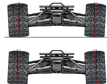
Positive camber
